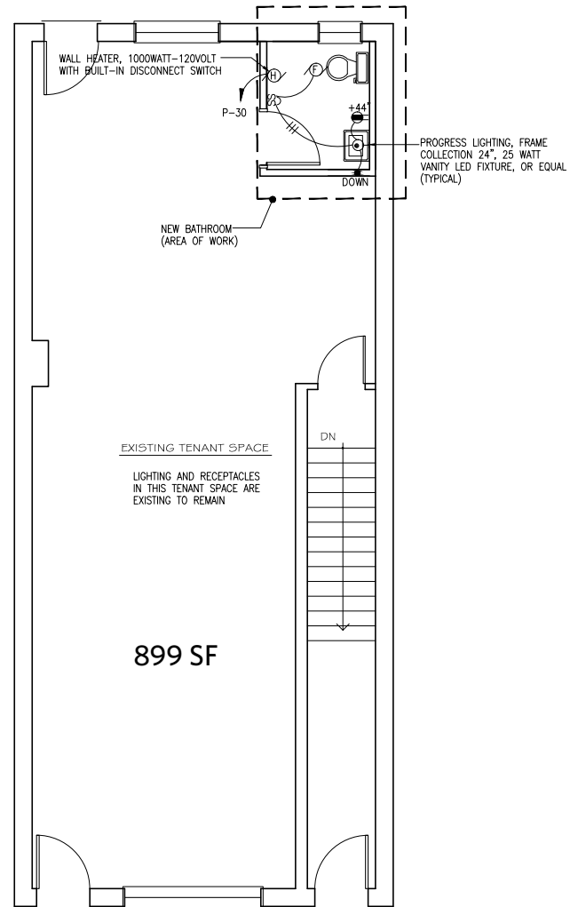
FIRST FLOOR PLAN-ELECTRICAL
