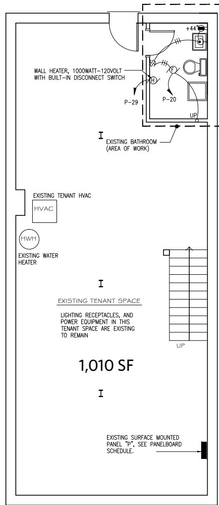
BASEMENT PLAN - ELECTRICAL
