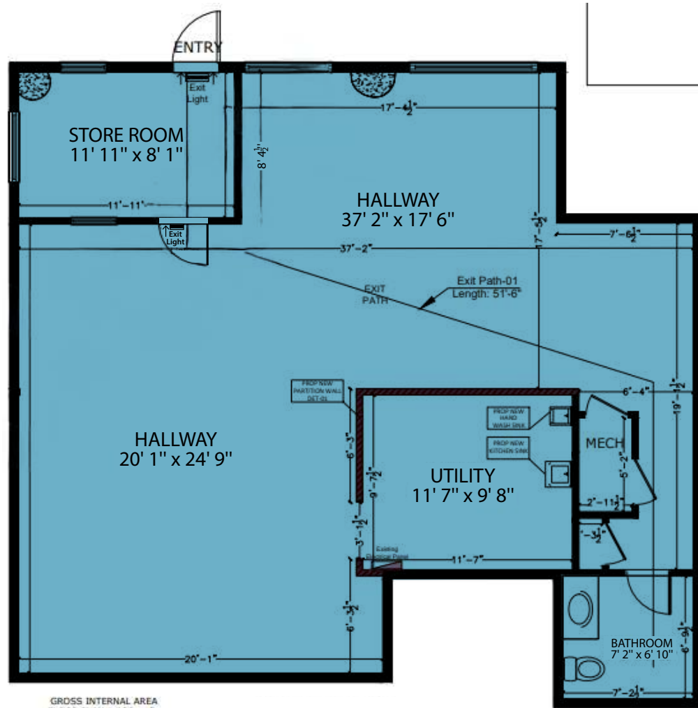
GROSS INTERNAL AREA FLOOR PLAN 1,126 sq.ft.
