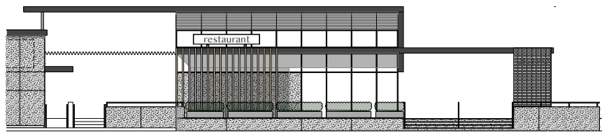
FRONT ELEVATION
